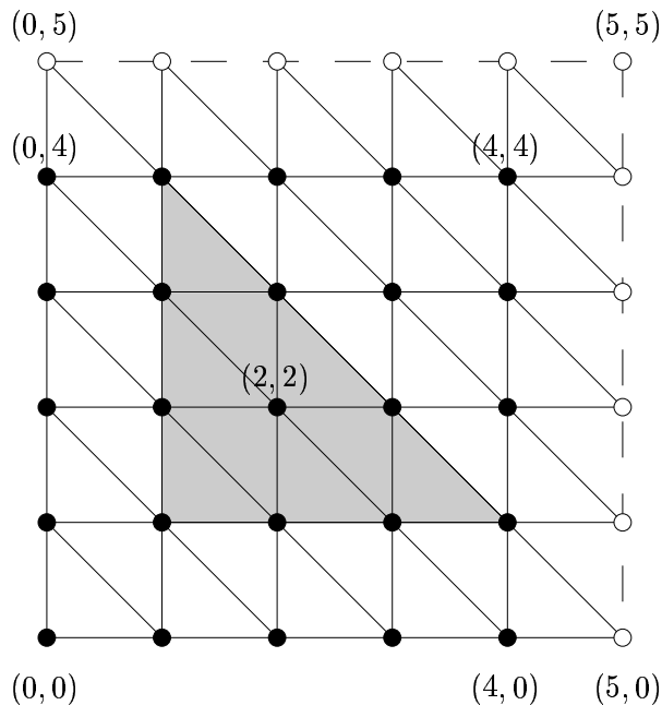
Figure 2: A torus T on \mathbb{Z}_5 \oplus \mathbb{Z}_5 .
