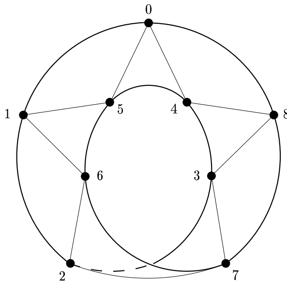
Figure 1: The Möbius band M = C_9(1, 4) .
